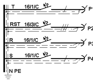
SCHEMA MONOFILARA
