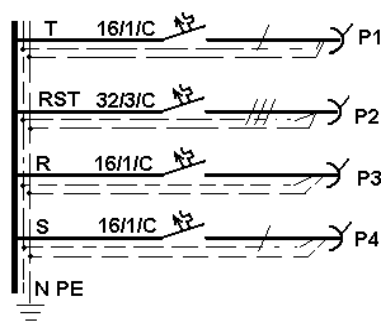
SCHEMA MONOFILARA
